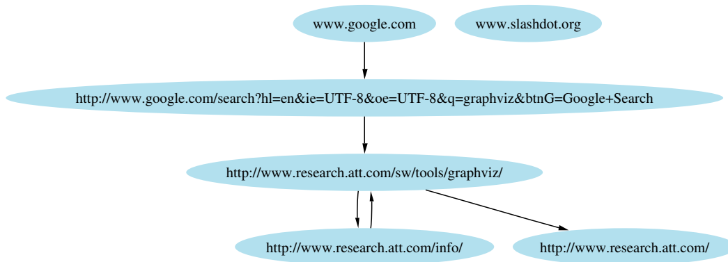
Figure 5: Complete URLs as labels in a history graph
