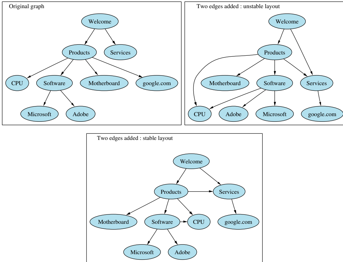
Figure 7: Unstable versus stable graph layout
